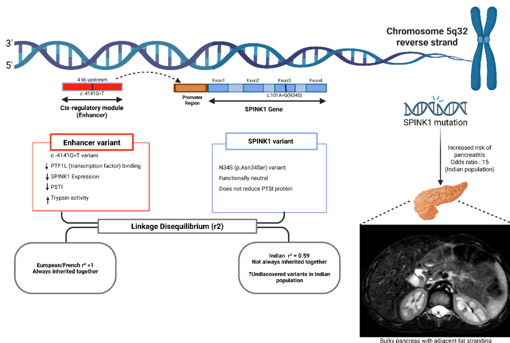
Figure 1: Genomic architecture and linkage disequilibrium of SPINK1 N34S haplotype.
